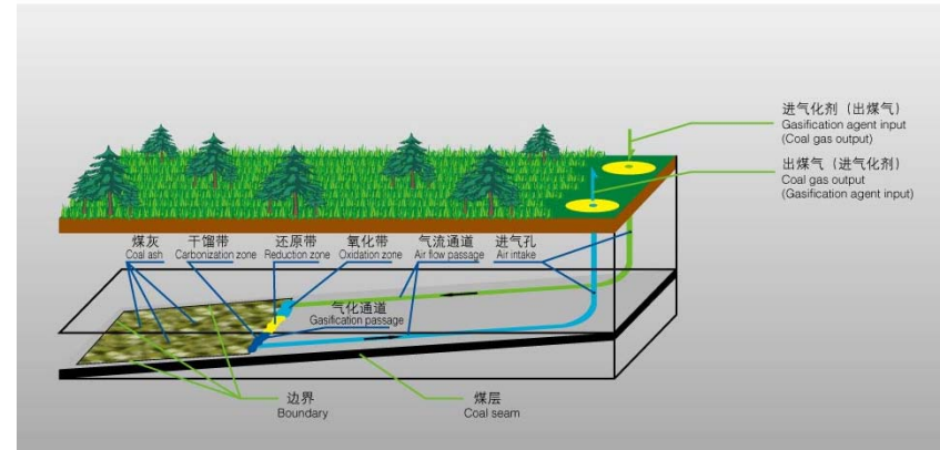
Underground Coal Gasification
