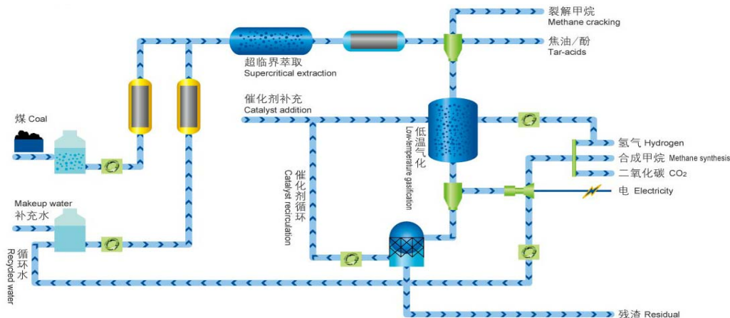
Catalytic Coal Gasification
